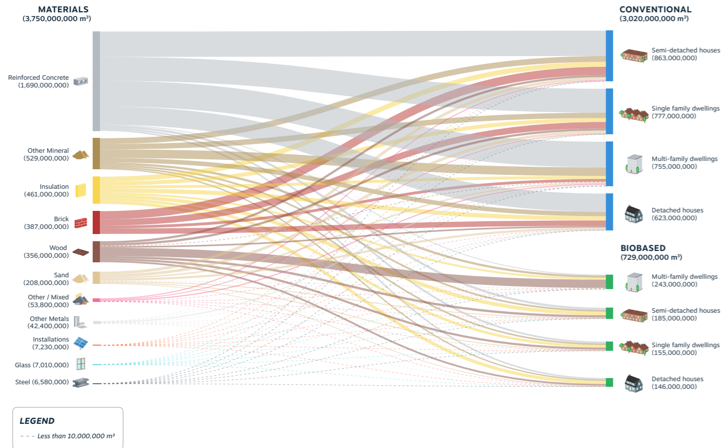
Figure 23 Cumulative Material Flow Analysis of High Ambition scenario, by volume (m³) until 2030.
